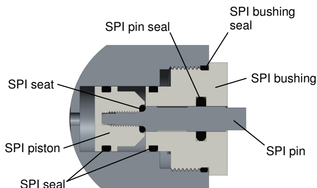
Set Point Indicator (SPI) (Optional)
